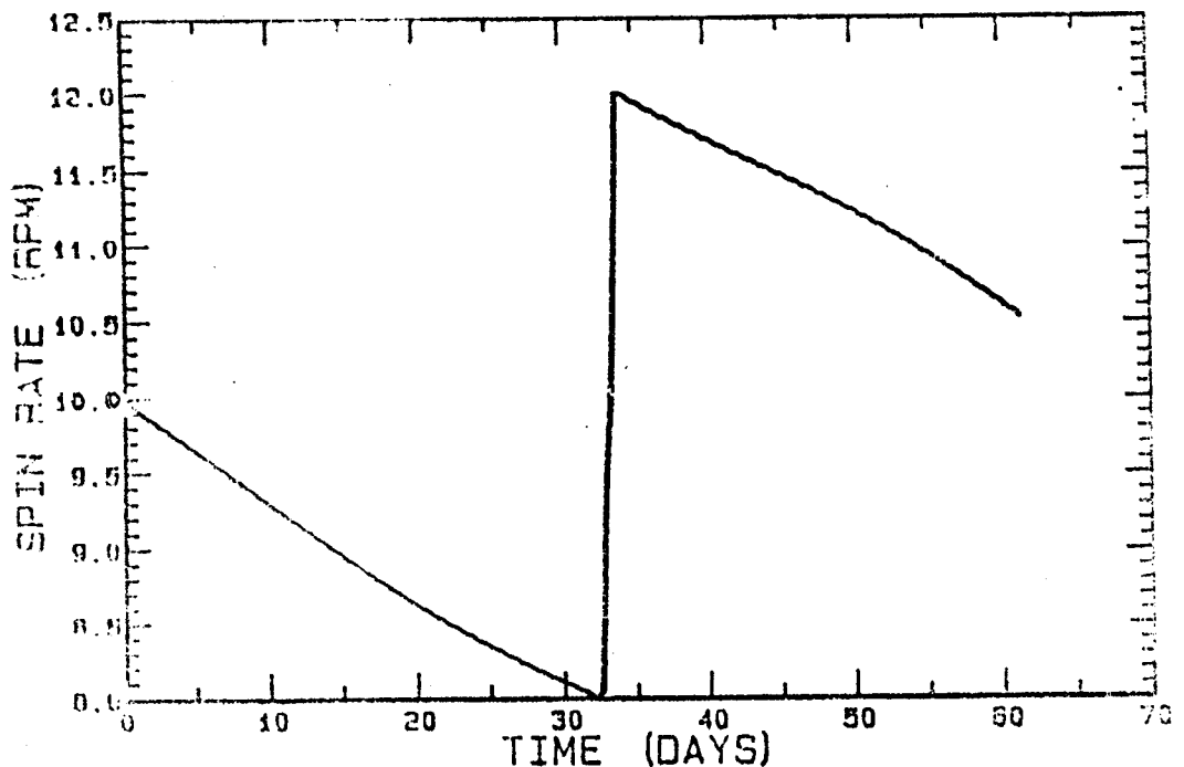
Fig. 3.6 - Spacecraft angular velocity before, during and after a spin rate maneuver.
