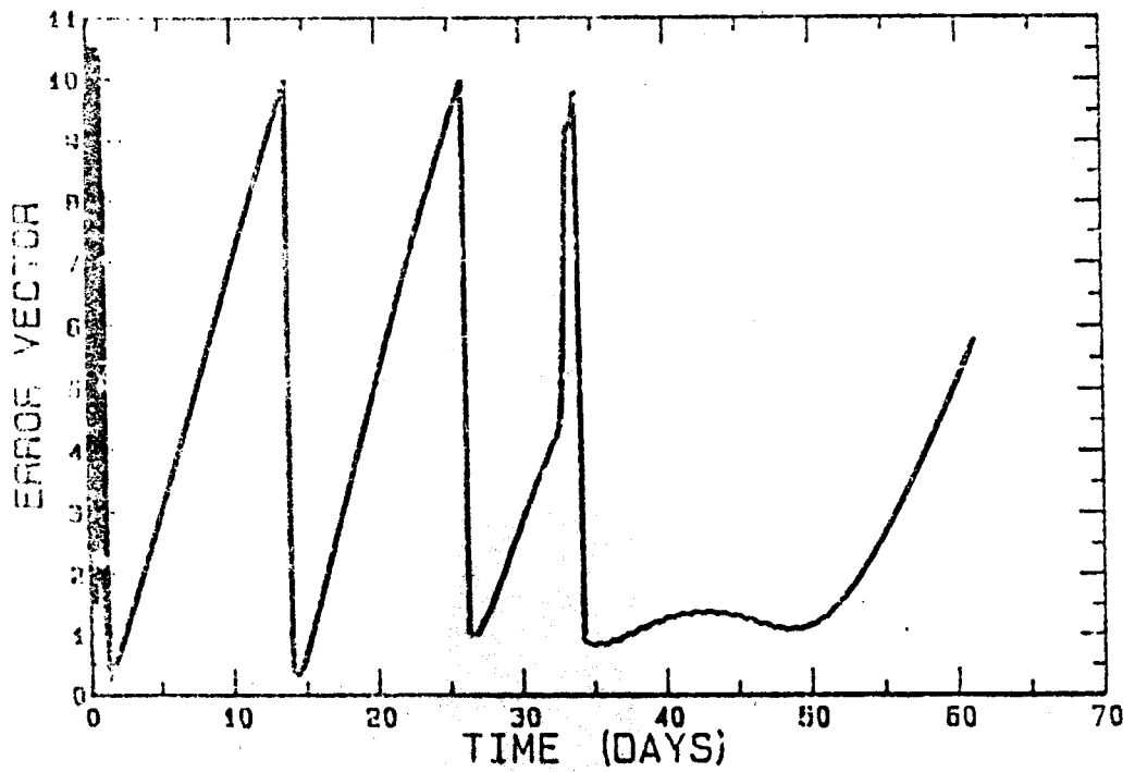
Fig. 3.4 - Error angle between the spin axis and the ecliptic normal.
